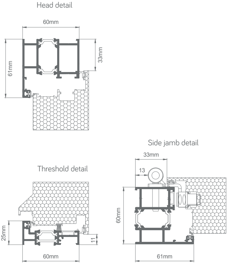
Smarts Signature Doors opening inwards
