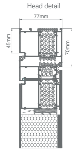
Head detail
