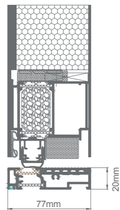
Threshold detail
