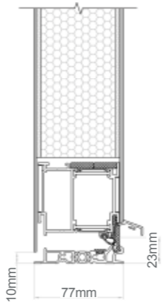
Threshold detail
