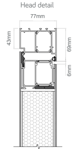
Head detail
